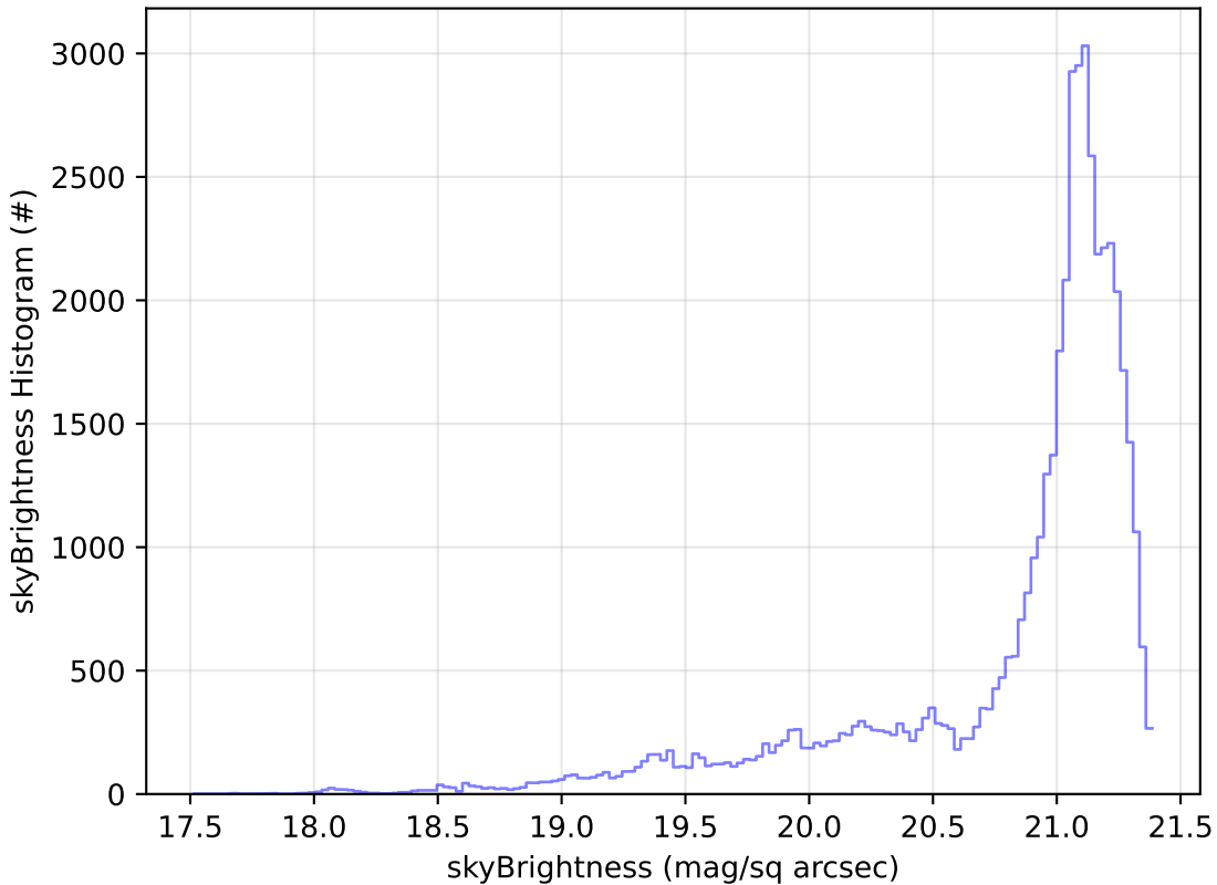
weather_cloudso0v3.4_10yrs Yr 1 r band: skyBrightness Histogram
