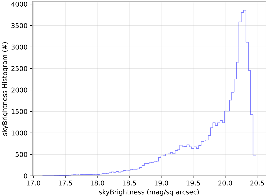
weather_cloudso0v3.4_10yrs Yr 1 i band: skyBrightness Histogram
