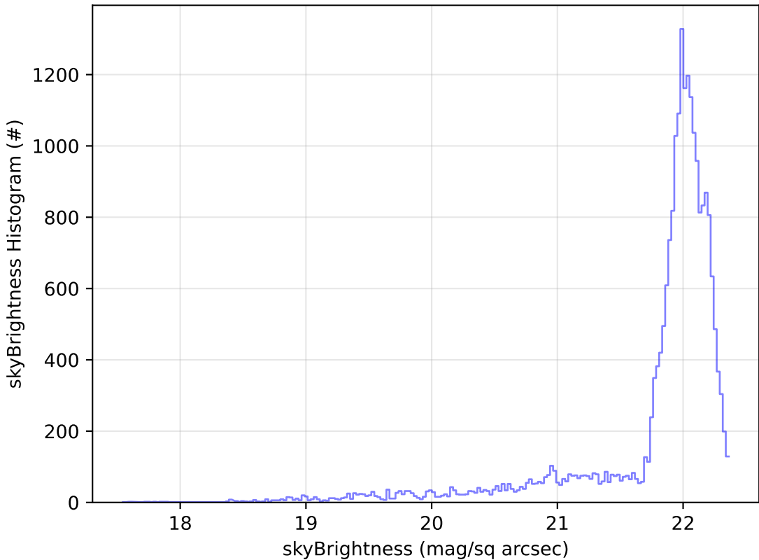
weather_cloudso0v3.4_10yrs Yr 1 g band: skyBrightness Histogram
