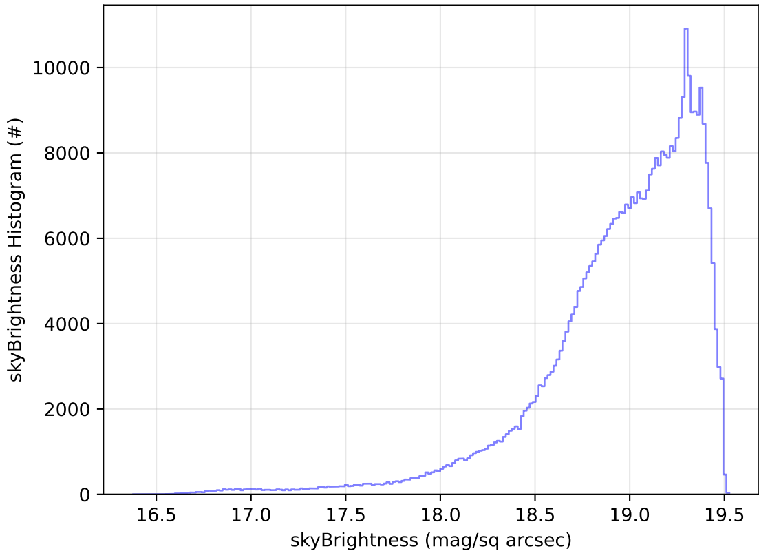
weather_cloudso0v3.4_10yrs WFD z band: skyBrightness Histogram
