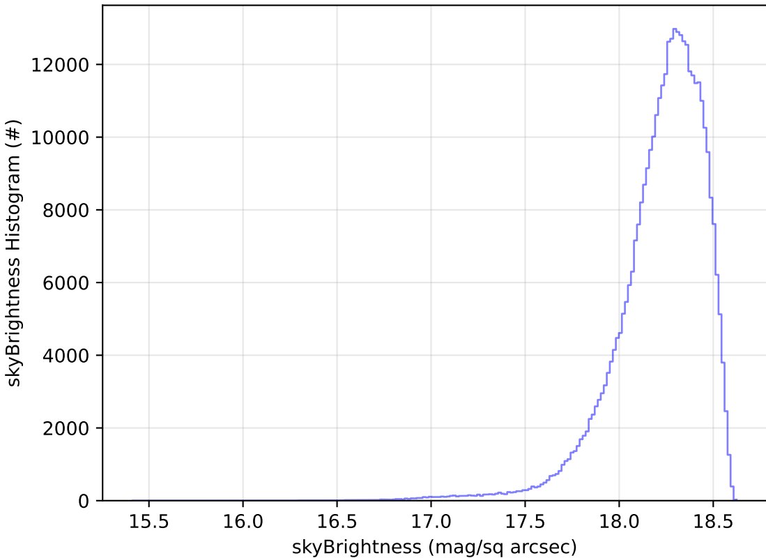
weather_cloudso0v3.4_10yrs WFD y band: skyBrightness Histogram
