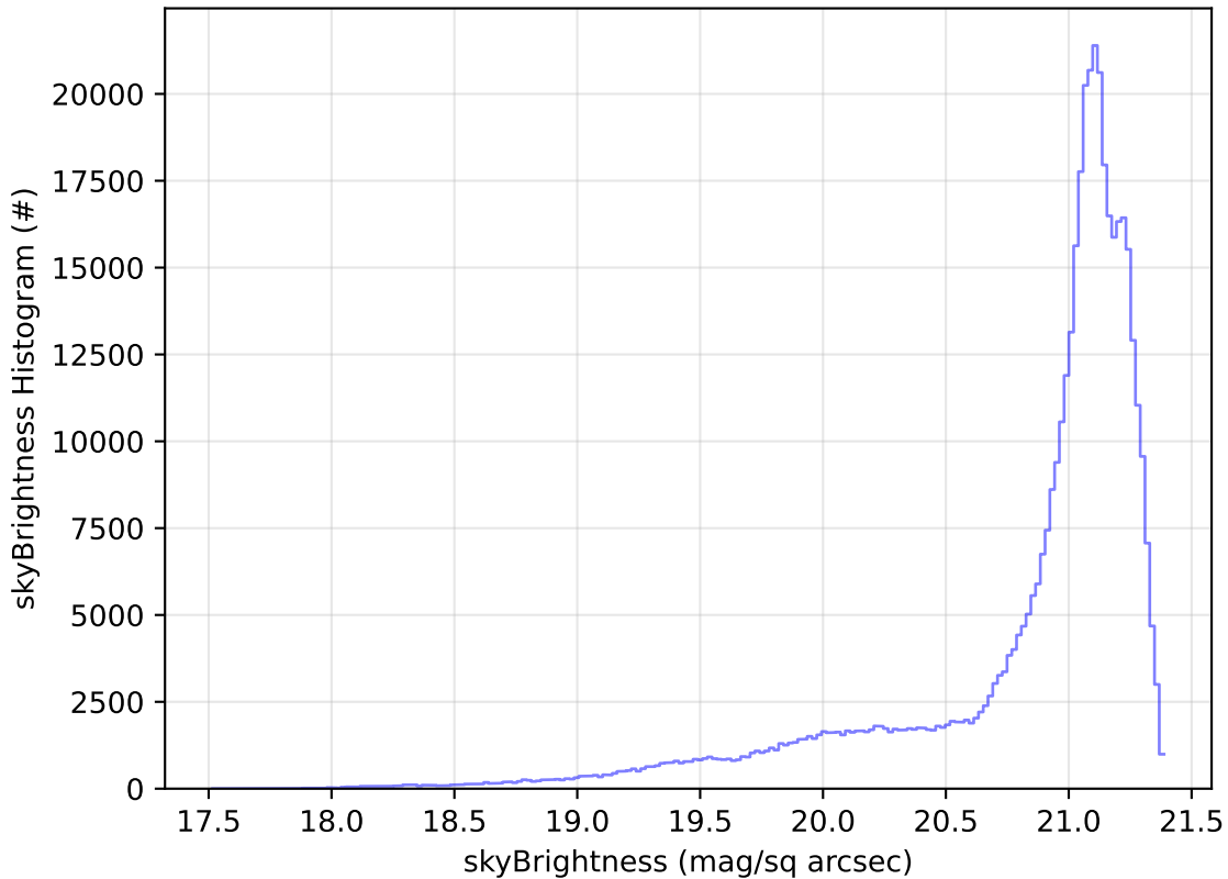
weather_cloudso0v3.4_10yrs WFD r band: skyBrightness Histogram
