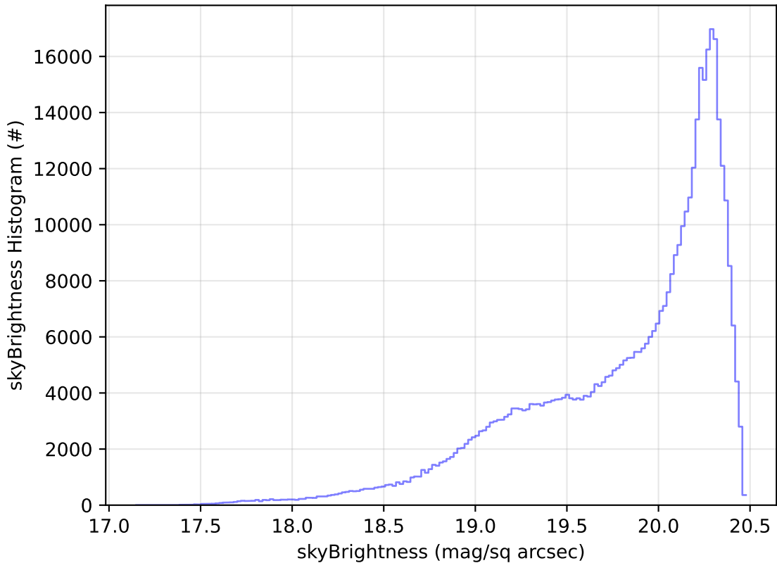
weather_cloudso0v3.4_10yrs WFD i band: skyBrightness Histogram
