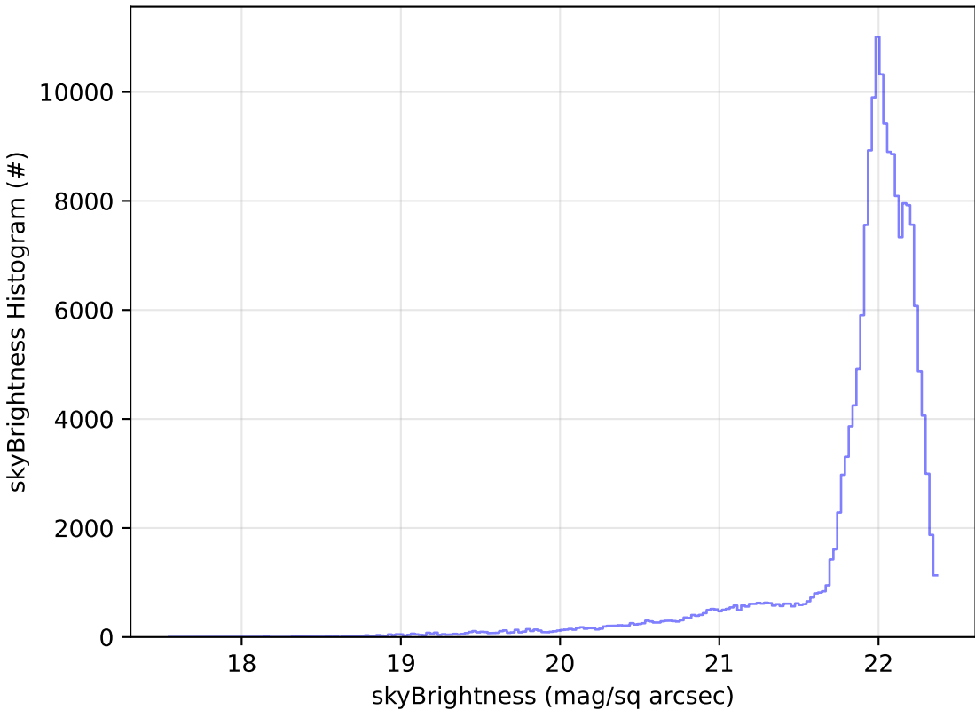
weather_cloudso0v3.4_10yrs WFD g band: skyBrightness Histogram
