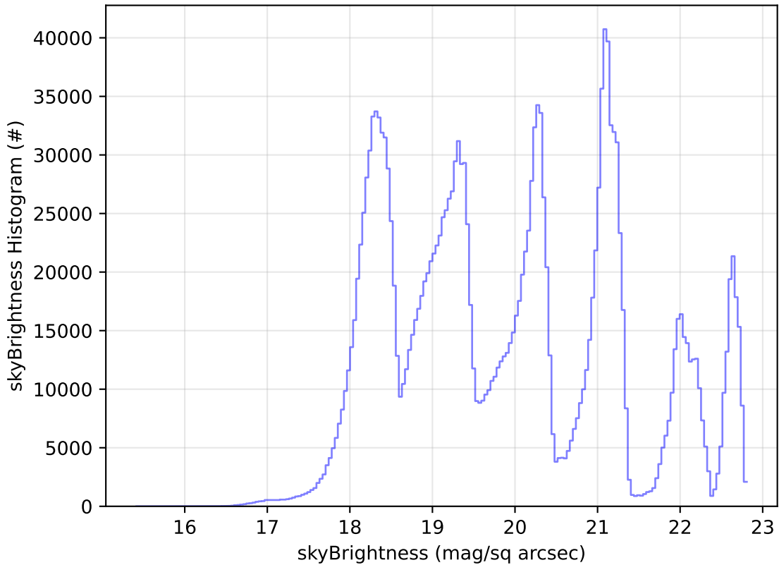
weather_cloudso0v3.4_10yrs WFD all bands: skyBrightness Histogram
