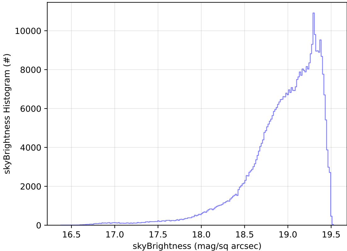
weather_cloudso0v3.4_10yrs All sky z band: skyBrightness Histogram
