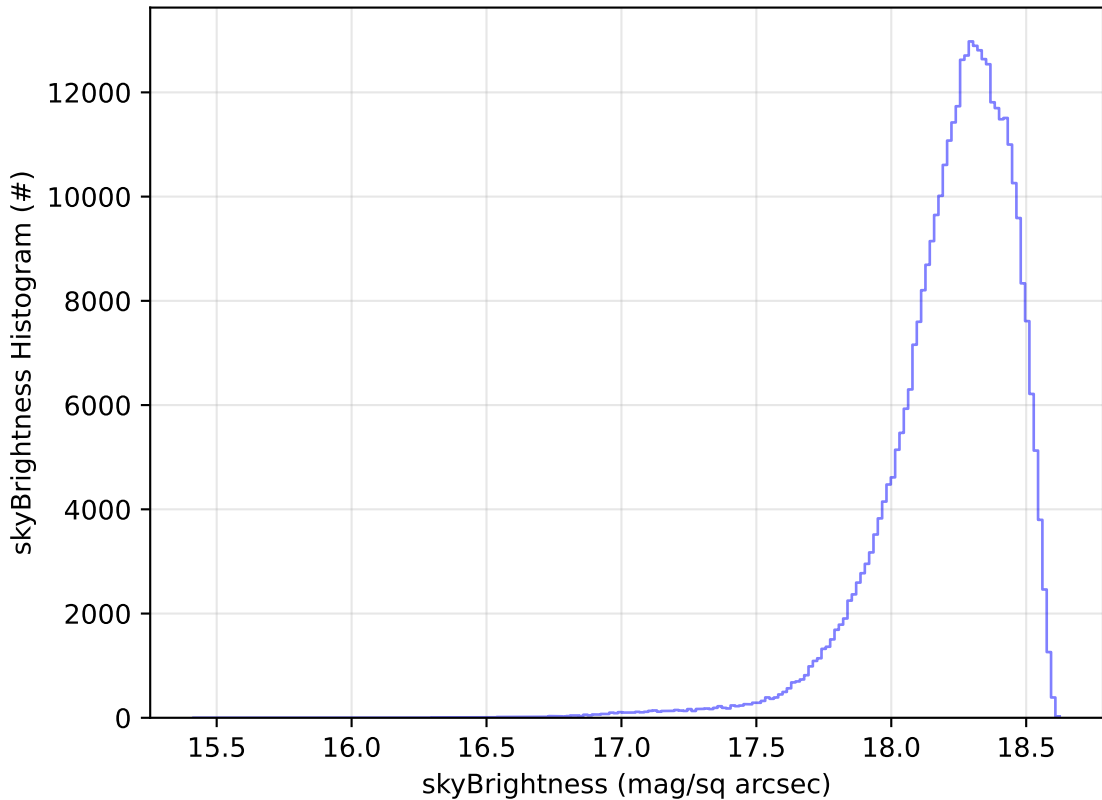
weather_cloudso0v3.4_10yrs All sky y band: skyBrightness Histogram
