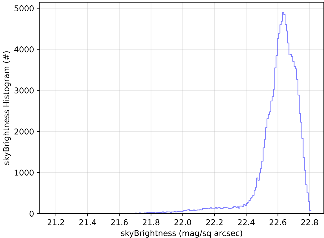
weather_cloudso0v3.4_10yrs All sky u band: skyBrightness Histogram
