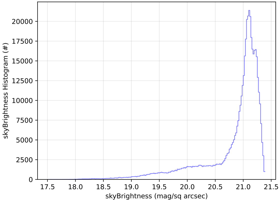
weather_cloudso0v3.4_10yrs All sky r band: skyBrightness Histogram
