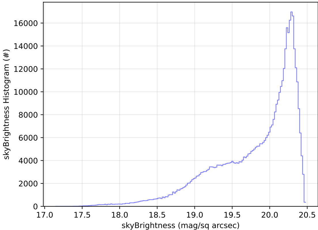
weather_cloudso0v3.4_10yrs All sky i band: skyBrightness Histogram
