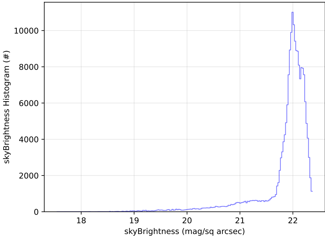
weather_cloudso0v3.4_10yrs All sky g band: skyBrightness Histogram
