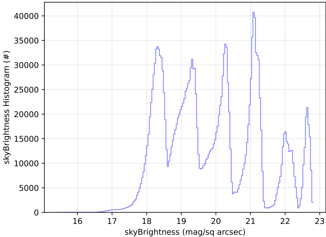
weather_cloudso0v3.4_10yrs All sky all bands: skyBrightness Histogram
