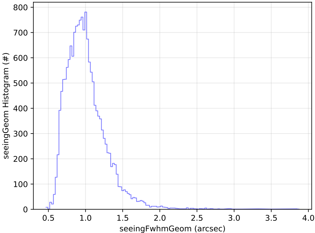
weather_cloudso0v3.4_10yrs Yr 1 u band: seeingGeom Histogram
