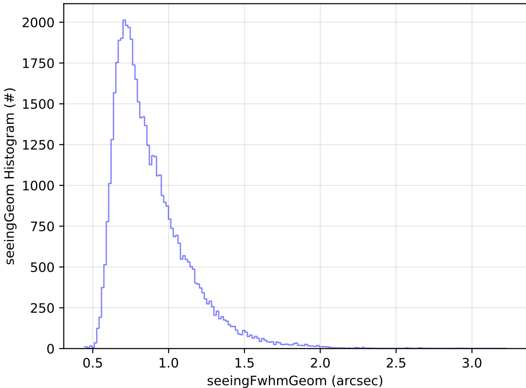
weather_cloudso0v3.4_10yrs Yr 1 r band: seeingGeom Histogram
