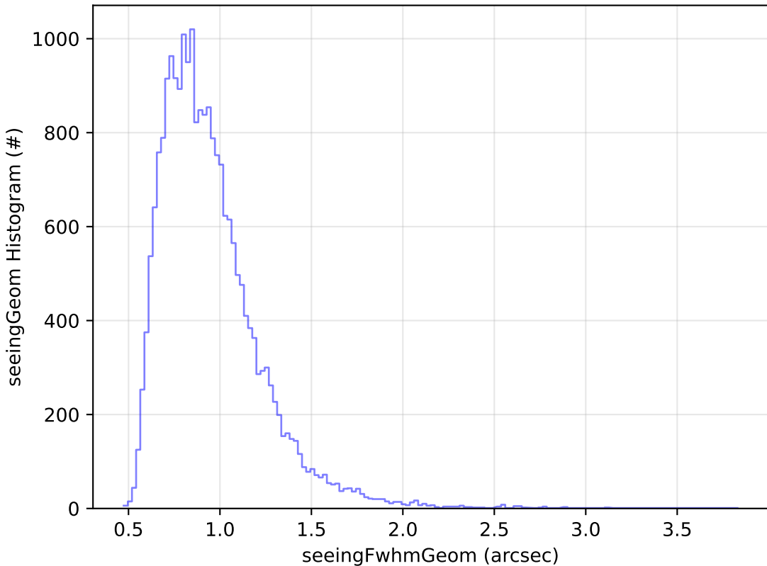
weather_cloudso0v3.4_10yrs Yr 1 g band: seeingGeom Histogram
