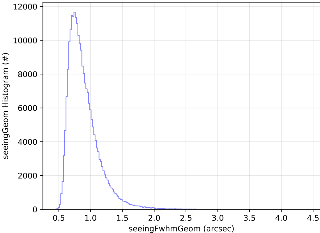
weather_cloudso0v3.4_10yrs Yr 1 all bands: seeingGeom Histogram
