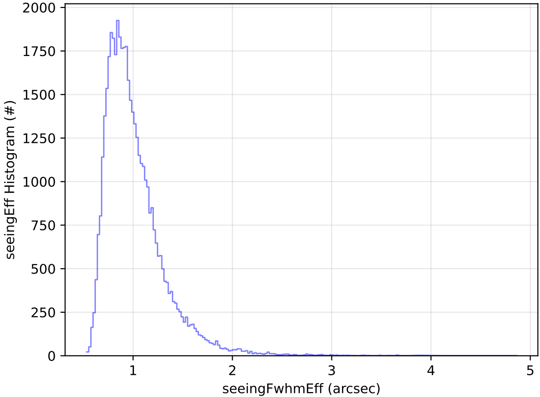
weather_cloudso0v3.4_10yrs Yr 1 z band: seeingEff Histogram
