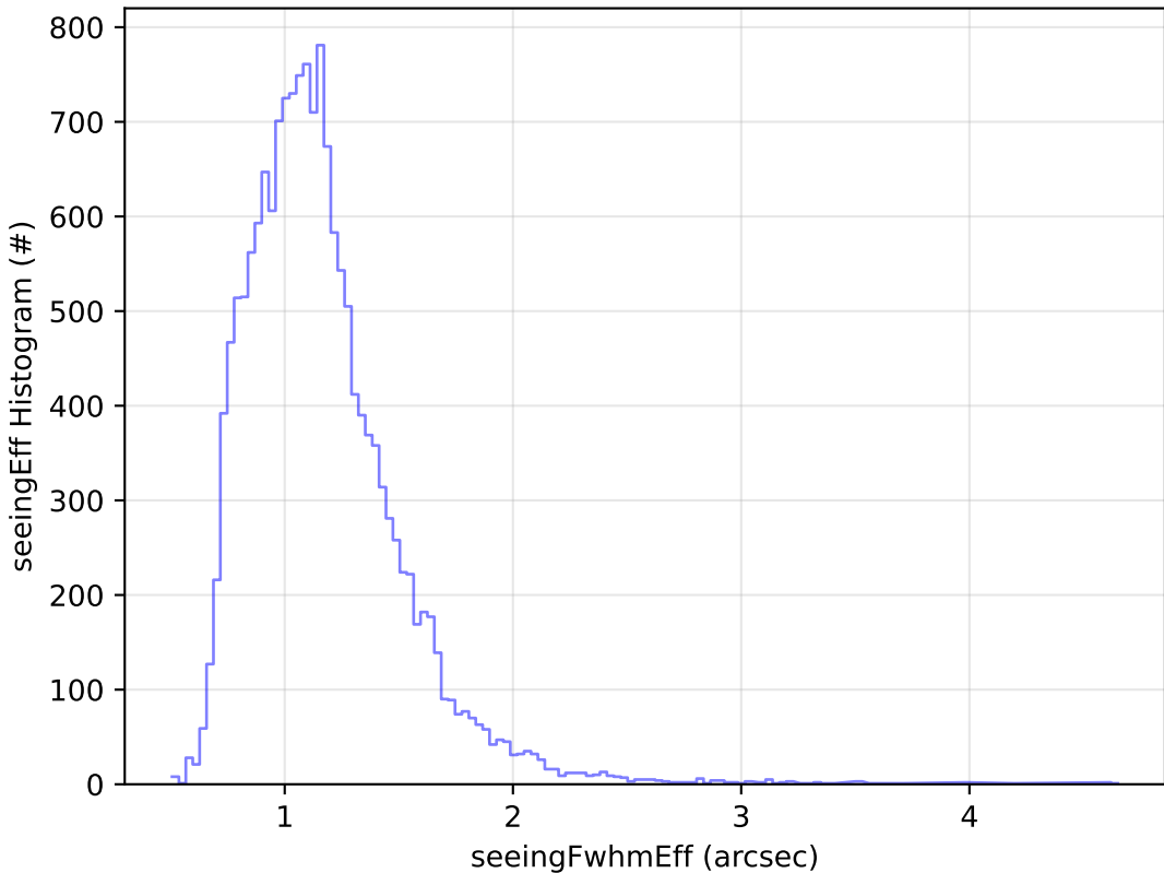
weather_cloudso0v3.4_10yrs Yr 1 u band: seeingEff Histogram
