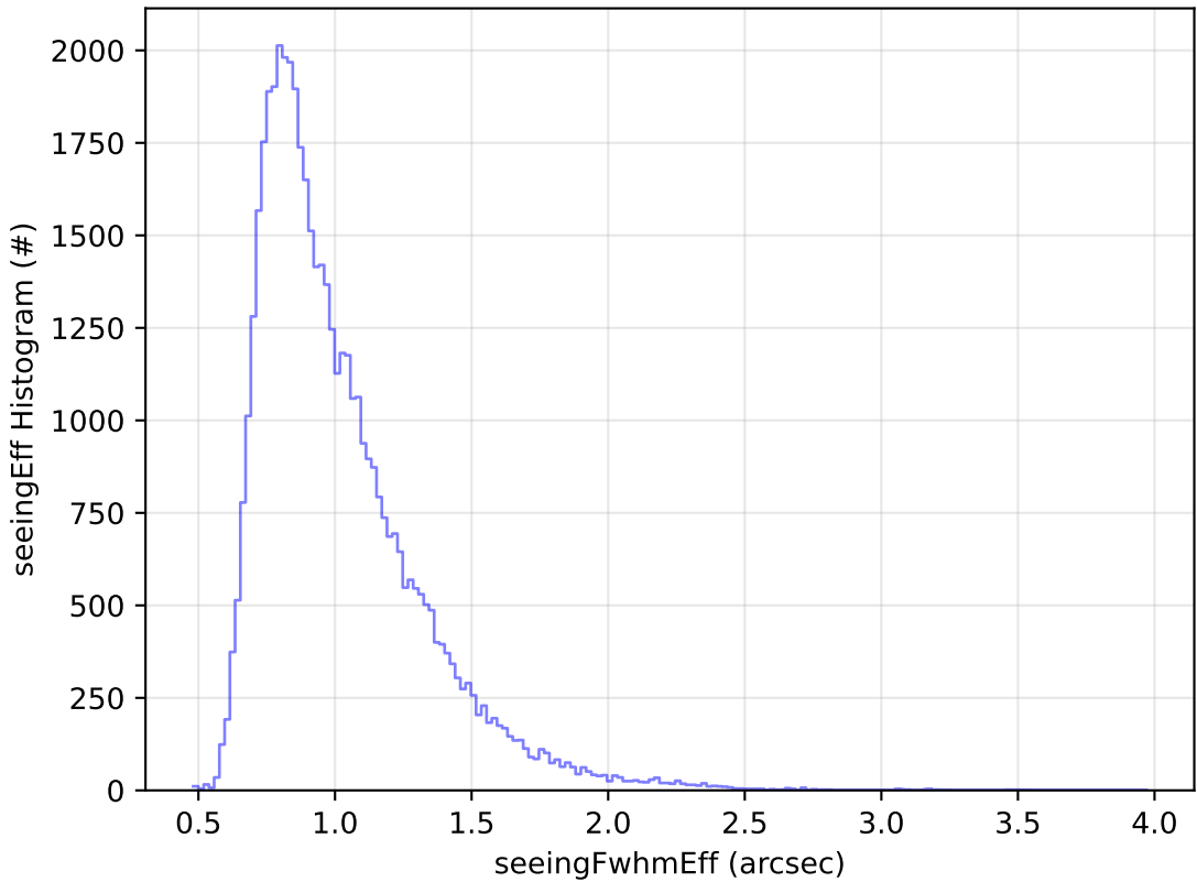
weather_cloudso0v3.4_10yrs Yr 1 r band: seeingEff Histogram
