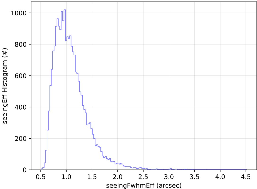
weather_cloudso0v3.4_10yrs Yr 1 g band: seeingEff Histogram
