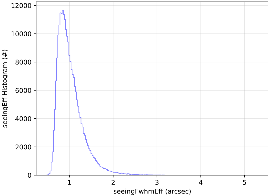
weather_cloudso0v3.4_10yrs Yr 1 all bands: seeingEff Histogram
