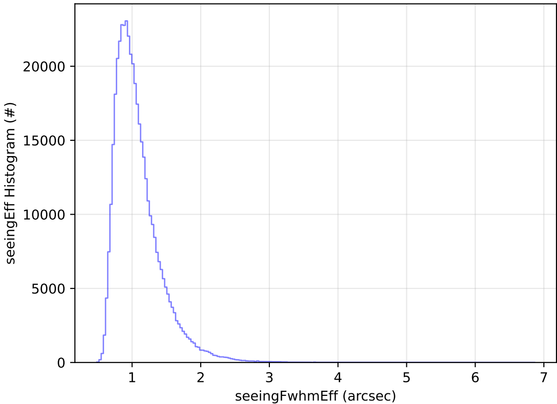
weather_cloudso0v3.4_10yrs WFD z band: seeingEff Histogram
