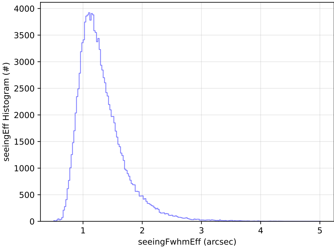
weather_cloudso0v3.4_10yrs WFD u band: seeingEff Histogram
