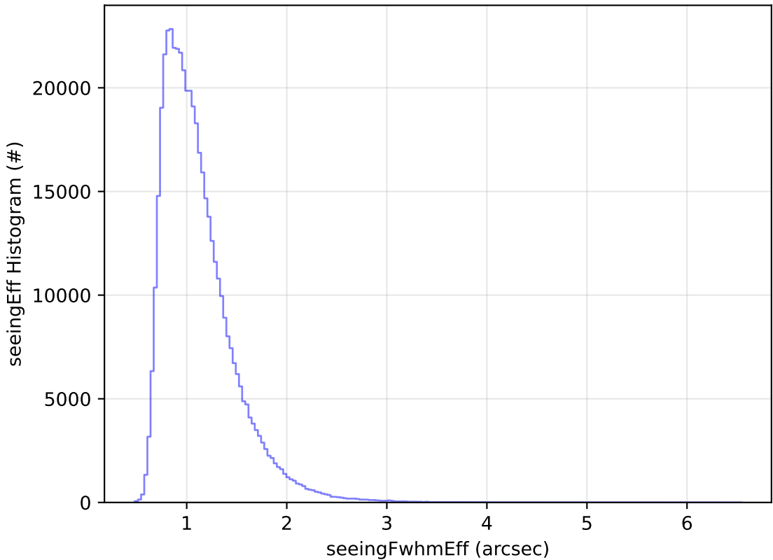
weather_cloudso0v3.4_10yrs WFD r band: seeingEff Histogram
