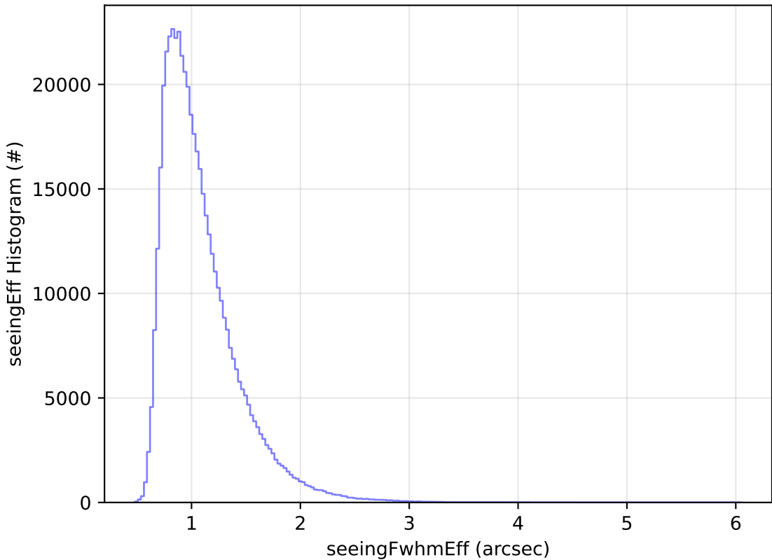
weather_cloudso0v3.4_10yrs WFD i band: seeingEff Histogram
