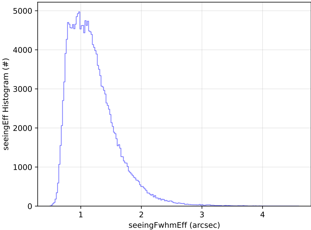
weather_cloudso0v3.4_10yrs WFD g band: seeingEff Histogram
