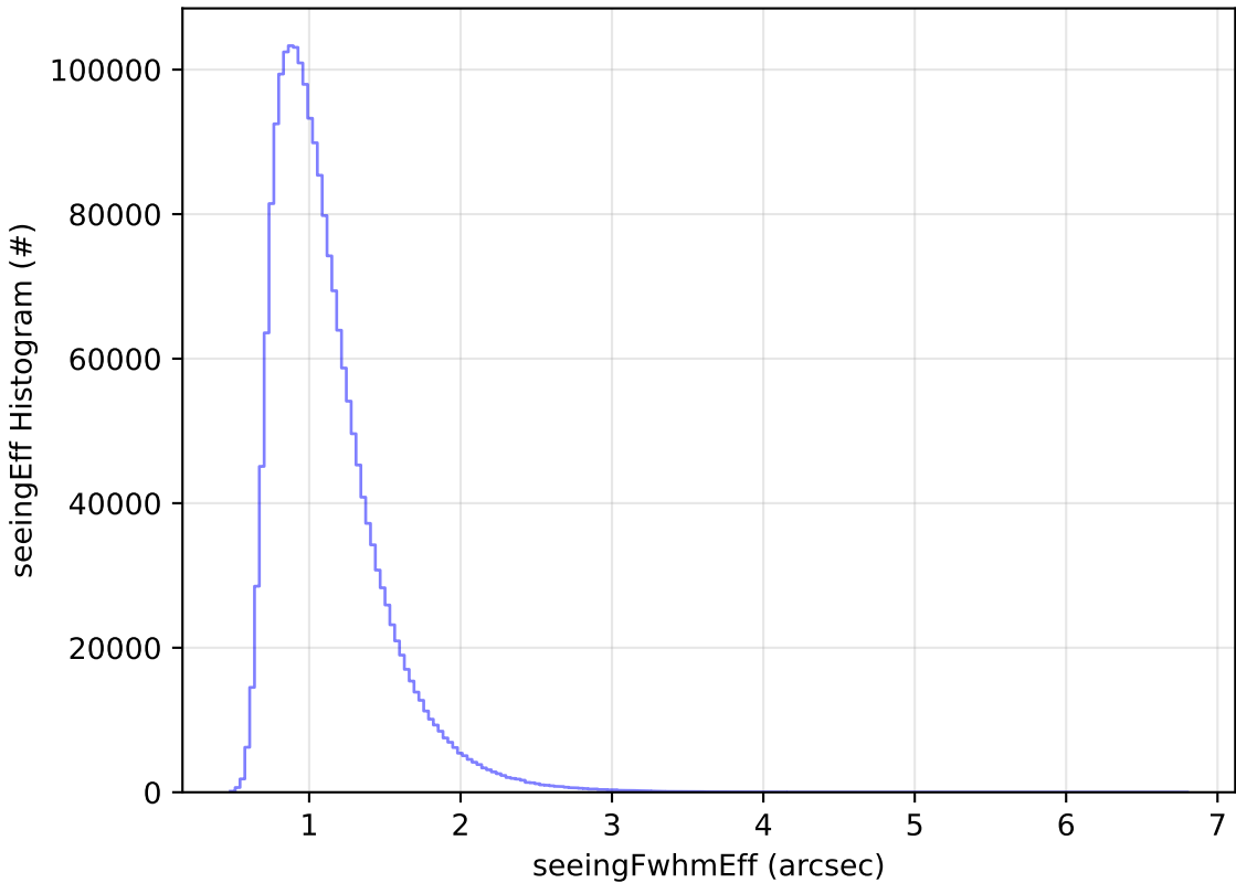
weather_cloudso0v3.4_10yrs WFD all bands: seeingEff Histogram
