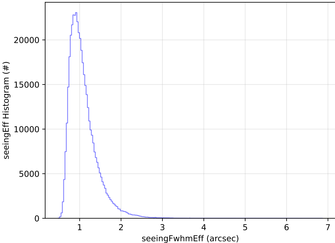
weather_cloudso0v3.4_10yrs All sky z band: seeingEff Histogram
