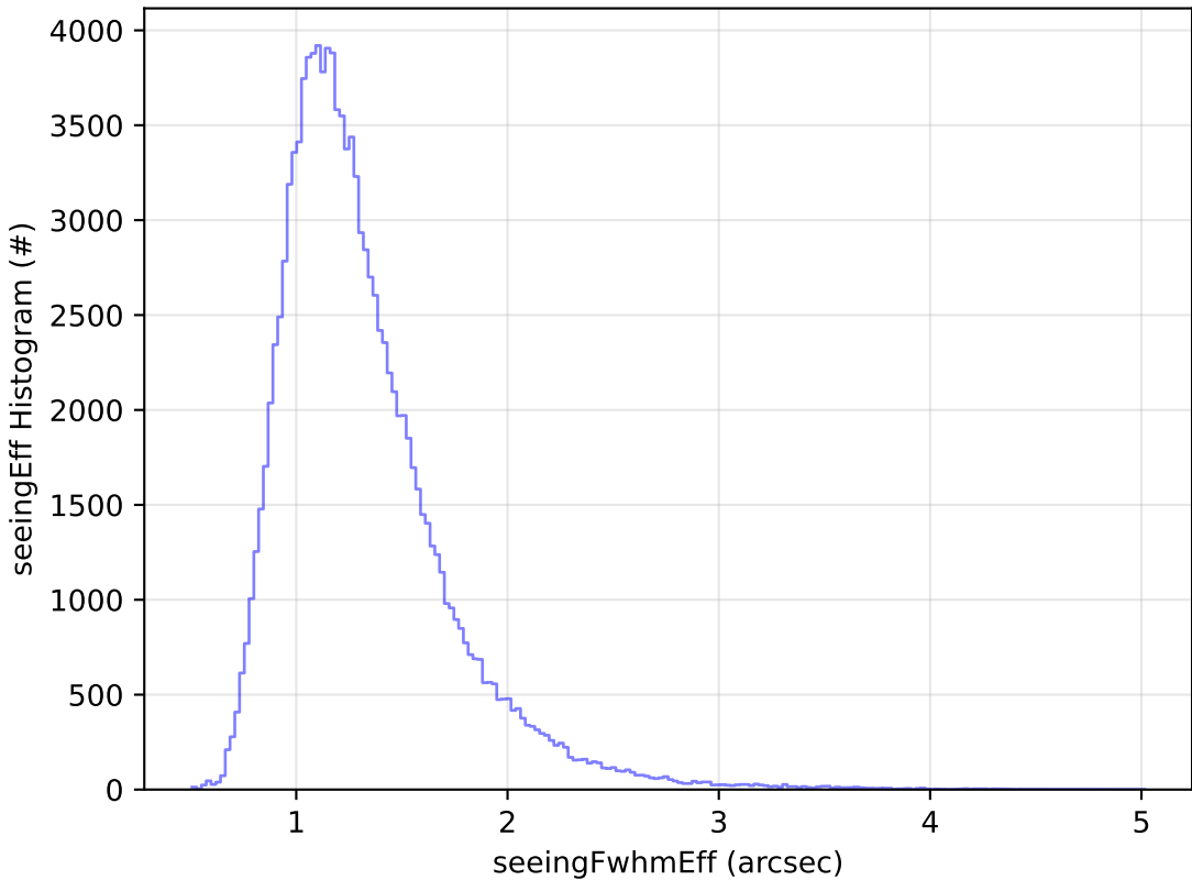
weather_cloudso0v3.4_10yrs All sky u band: seeingEff Histogram
