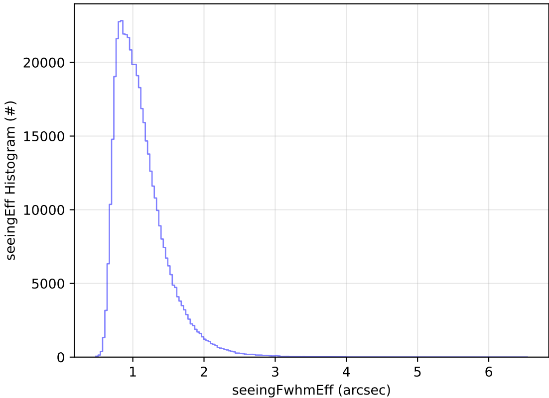
weather_cloudso0v3.4_10yrs All sky r band: seeingEff Histogram
