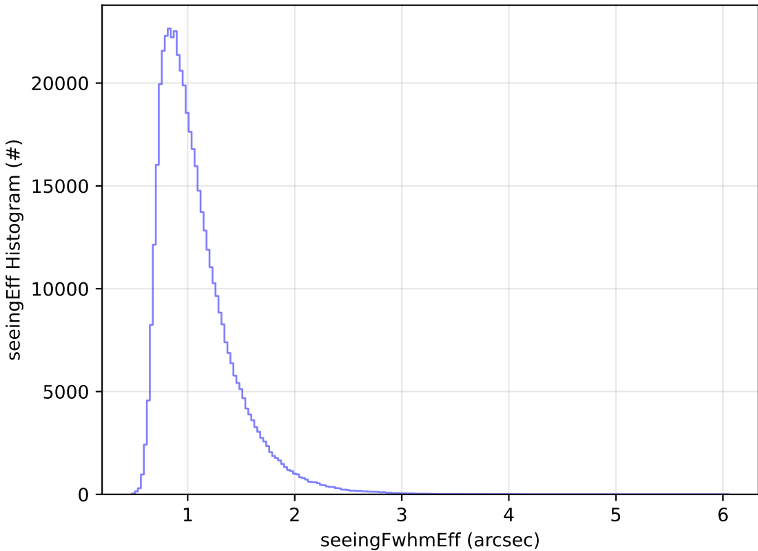
weather_cloudso0v3.4_10yrs All sky i band: seeingEff Histogram
