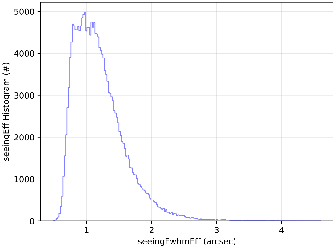
weather_cloudso0v3.4_10yrs All sky g band: seeingEff Histogram
