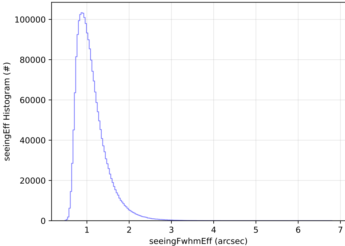
weather_cloudso0v3.4_10yrs All sky all bands: seeingEff Histogram
