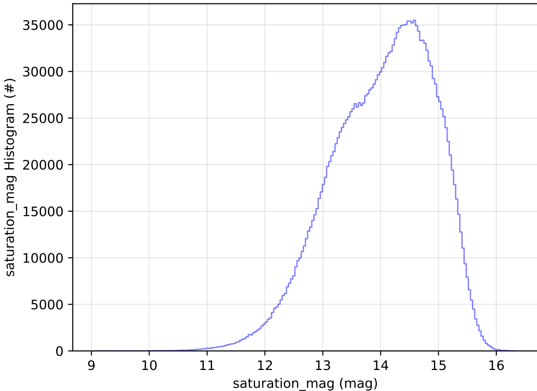
weather_cloudso0v3.4_10yrs WFD all bands: saturation_mag Histogram
