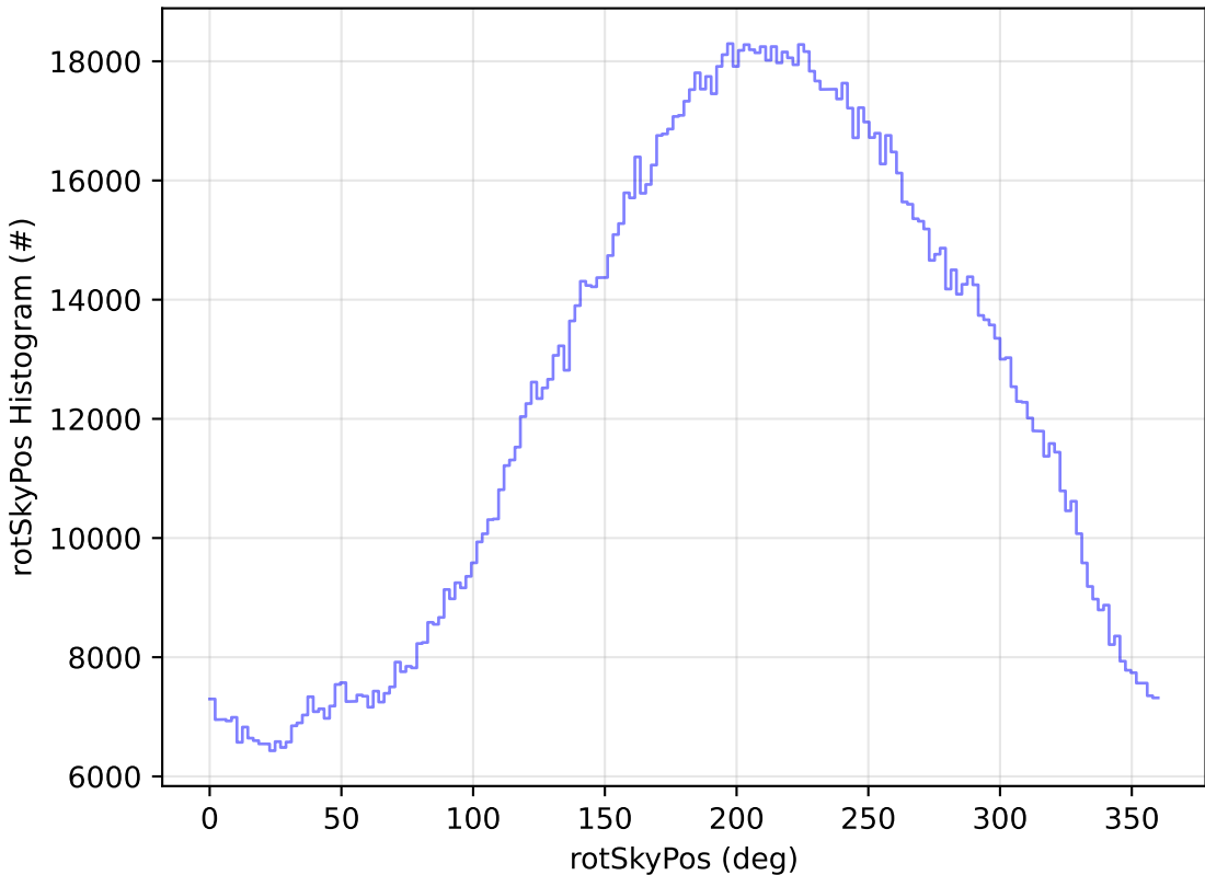
weather_cloudso0v3.4_10yrs WFD all bands: rotSkyPos Histogram
