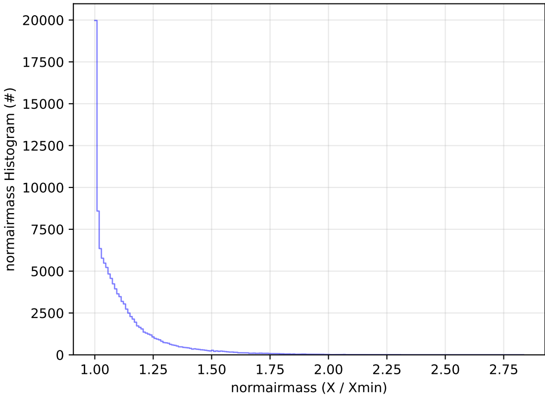
weather_cloudso0v3.4_10yrs WFD u band: normairmass Histogram
