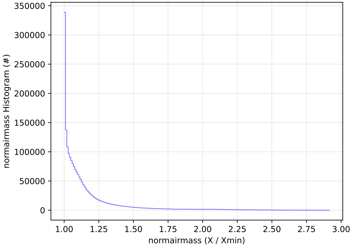
weather_cloudso0v3.4_10yrs WFD all bands: normairmass Histogram
