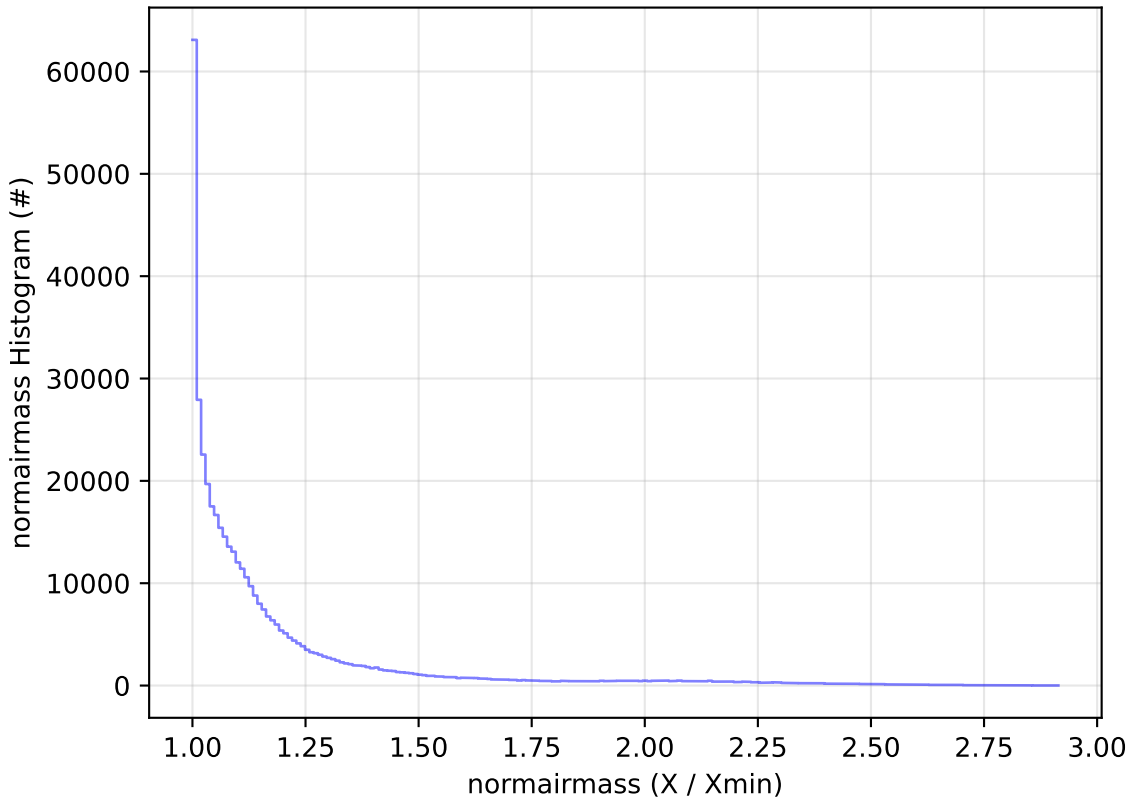
weather_cloudso0v3.4_10yrs All sky z band: normairmass Histogram
