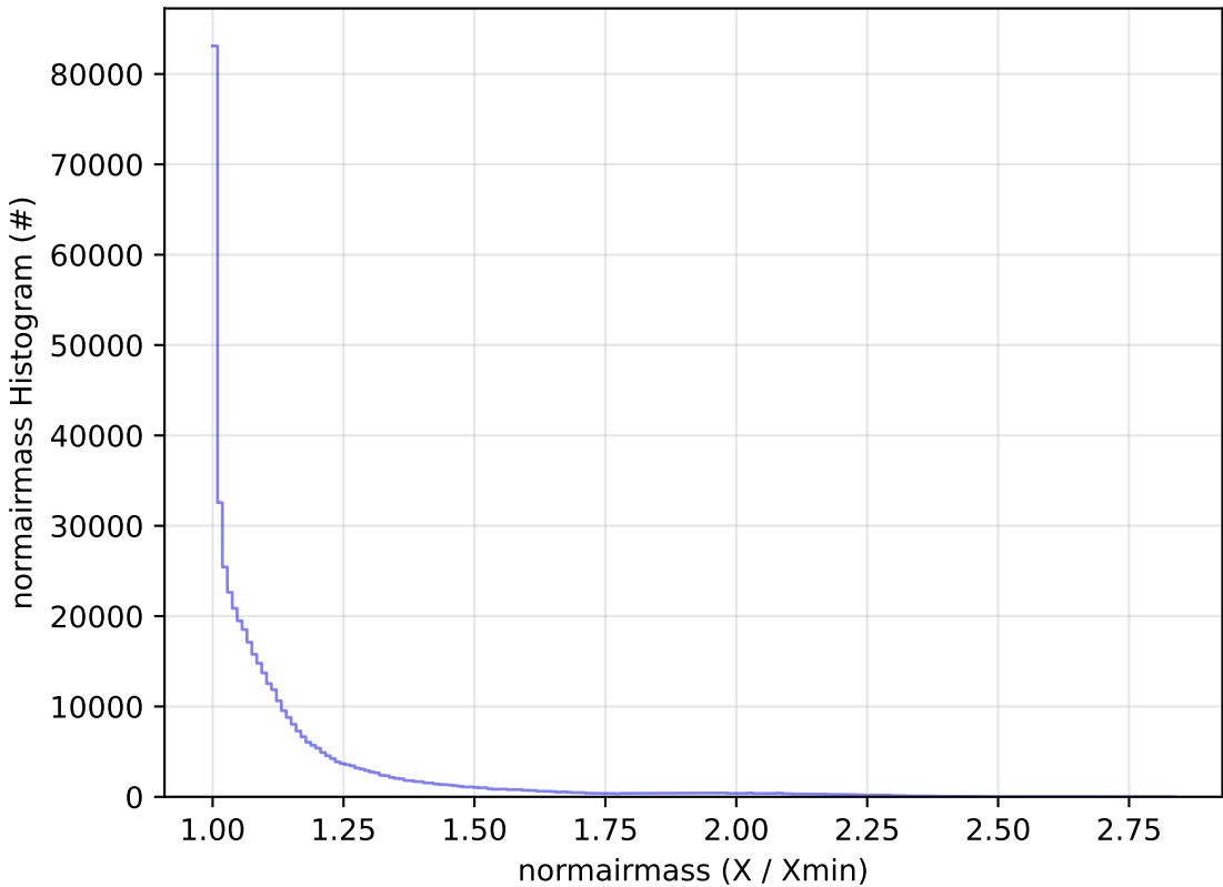
weather_cloudso0v3.4_10yrs All sky r band: normairmass Histogram
