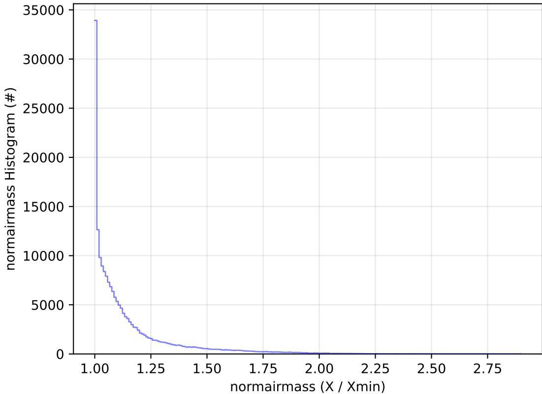
weather_cloudso0v3.4_10yrs All sky g band: normairmass Histogram
