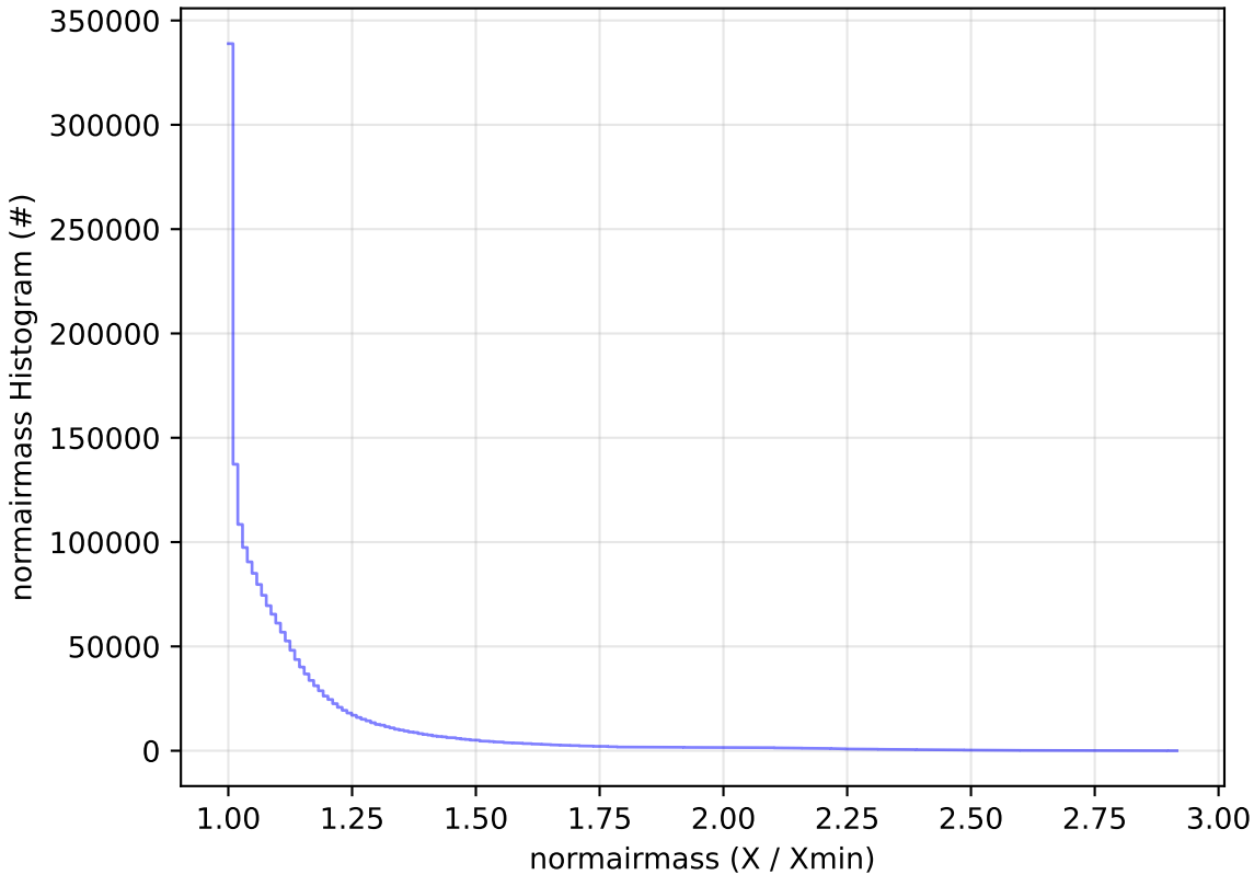
weather_cloudso0v3.4_10yrs All sky all bands: normairmass Histogram
