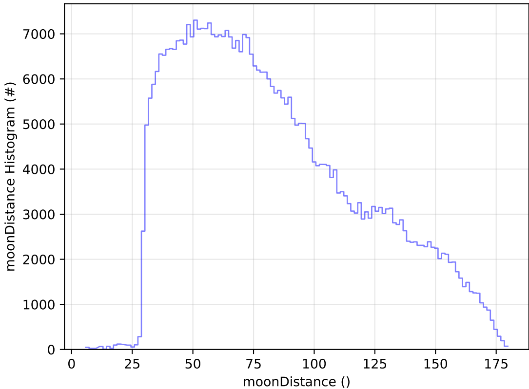
weather_cloudso0v3.4_10yrs WFD z band: moonDistance Histogram
