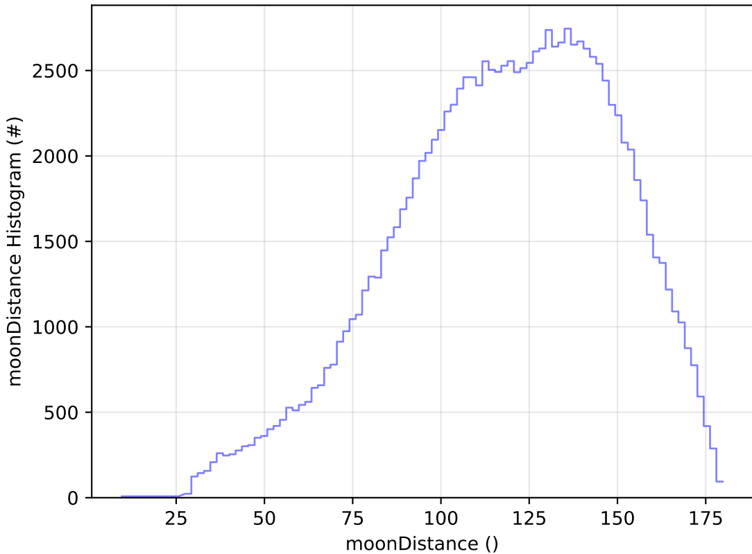
weather_cloudso0v3.4_10yrs WFD u band: moonDistance Histogram
