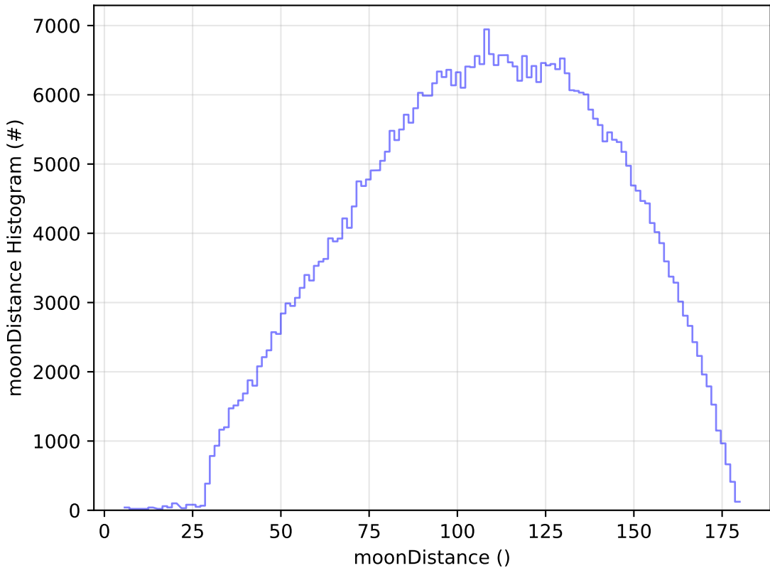
weather_cloudso0v3.4_10yrs WFD r band: moonDistance Histogram
