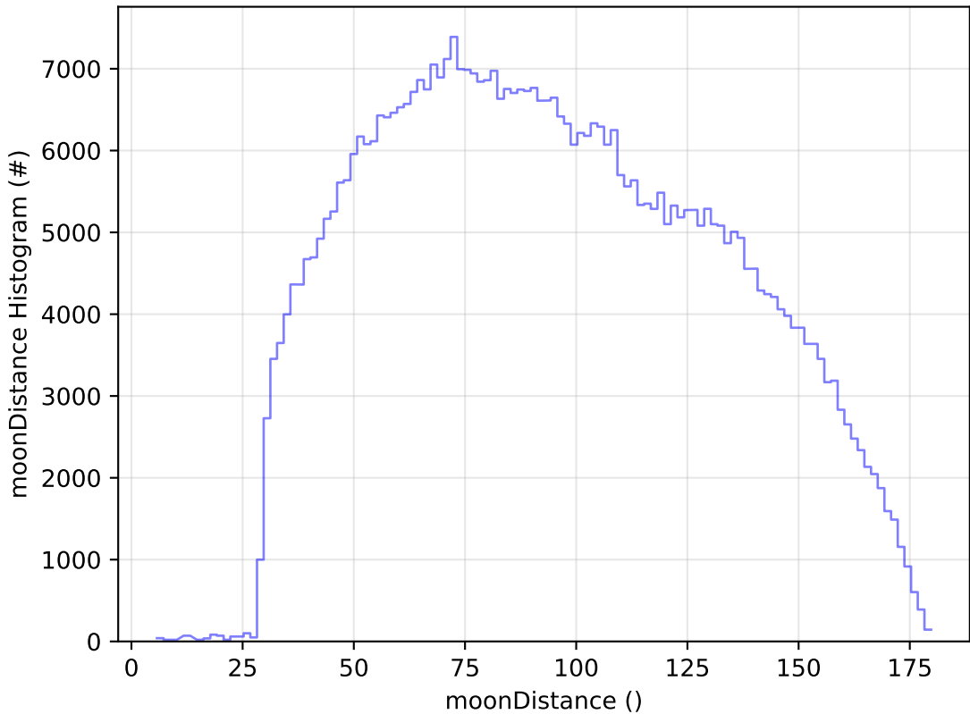
weather_cloudso0v3.4_10yrs WFD i band: moonDistance Histogram
