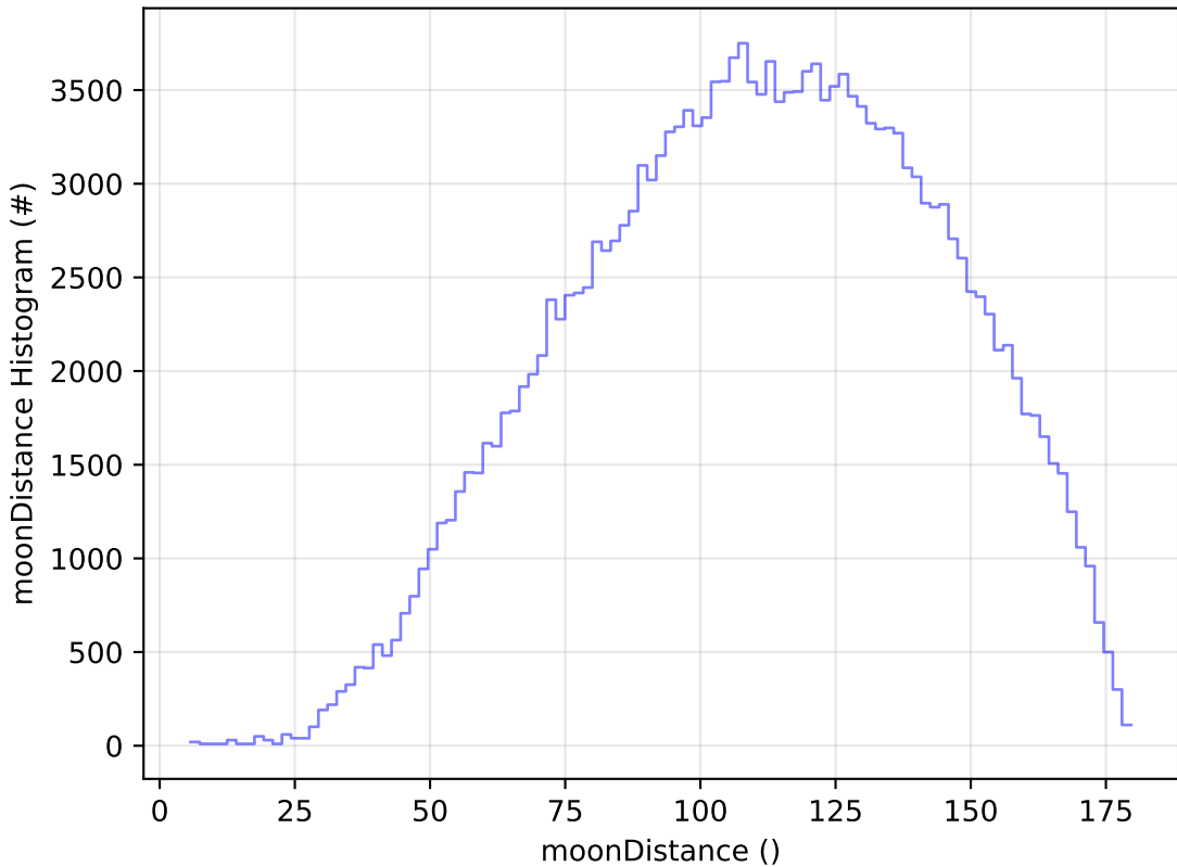
weather_cloudso0v3.4_10yrs WFD g band: moonDistance Histogram
